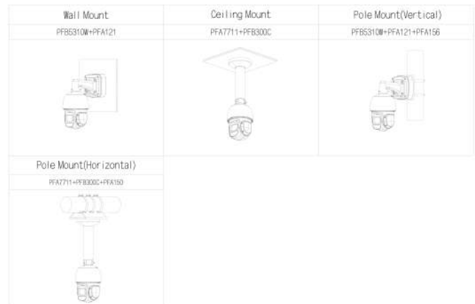
DH-PFA156 Pole Mount Bracket
